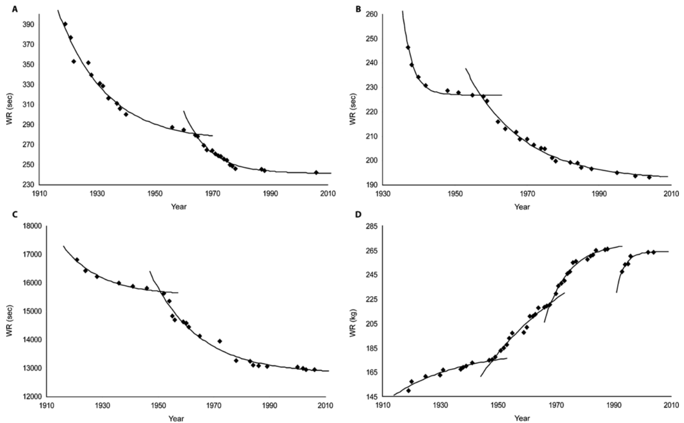
Figure 1. Model fitting on 4 events. A. Women 400 m freestyle (swimming) with biexponential decaying curve, adjusted r_i^2=0.976 and r_{ii}^2=0.966 ; B. Men 4x100 m freestyle relay (swimming), r_i^2=0.985 , r_{ii}^2=0.988 ; C. Men 50 km walk (track), r_i^2=0.972 , r_{ii}^2=0.977 ; D. Clean & Jerk Super Heavyweight (weight lifting), r_i^2=0.939 , r_{ii}^2=0.937 , r_{iii}^2=0.975 and r_{iv}^2=0.946 . Weight categories were altered in 1948, 1968 and 1992 and control reinforced in 1988–1992 in weight lifting. doi:10.1371/journal.pone.0001552.g001
